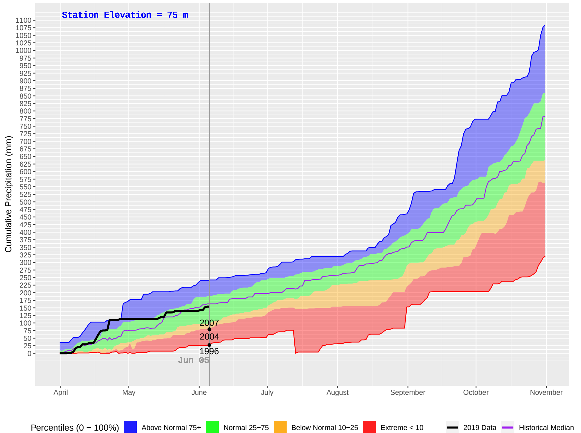
KITPARK (106) : Historical (1995–2018), Current (2019) Daily Cumulative Precipitation
