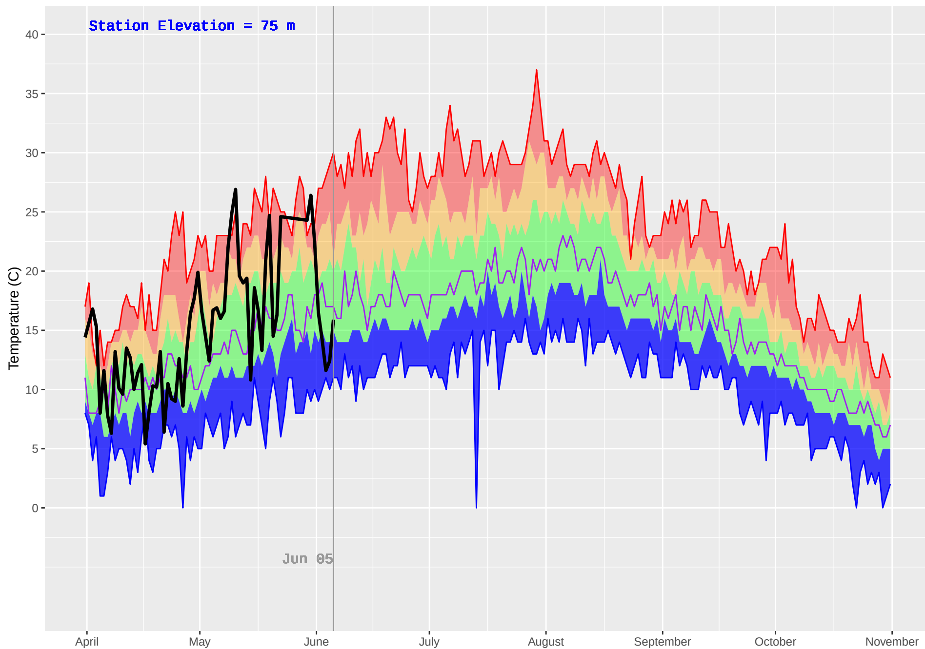
KITPARK (106) : Historical (1995–2018) and Current (2019) Daily Temperature
