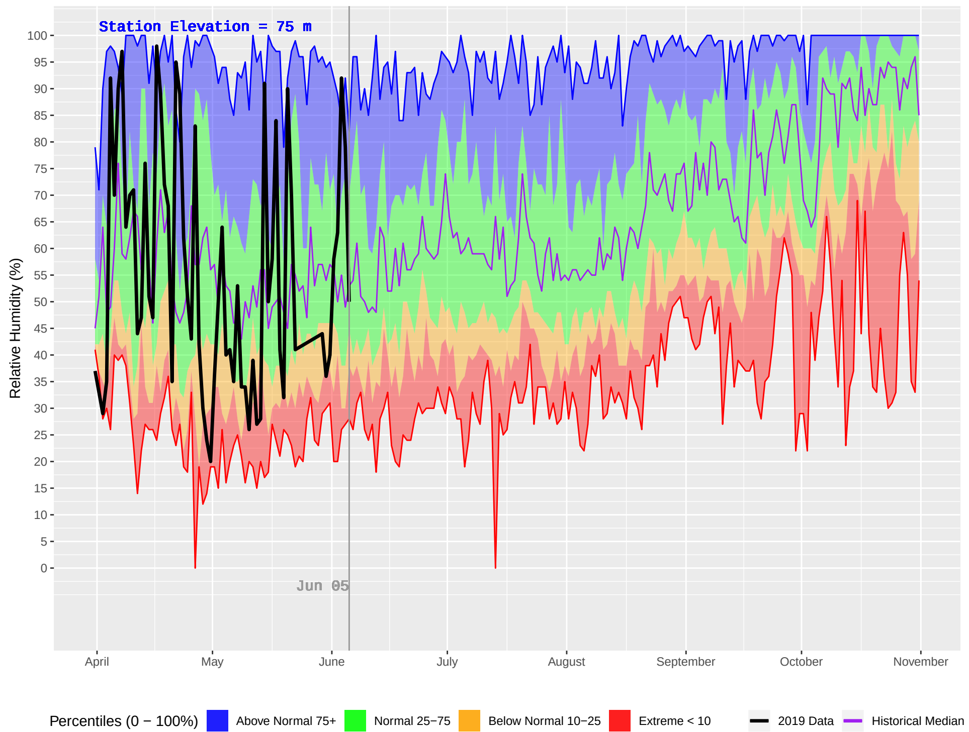
KITPARK (106) : Historical (1995–2018) and Current (2019) Daily Relative Humidity
