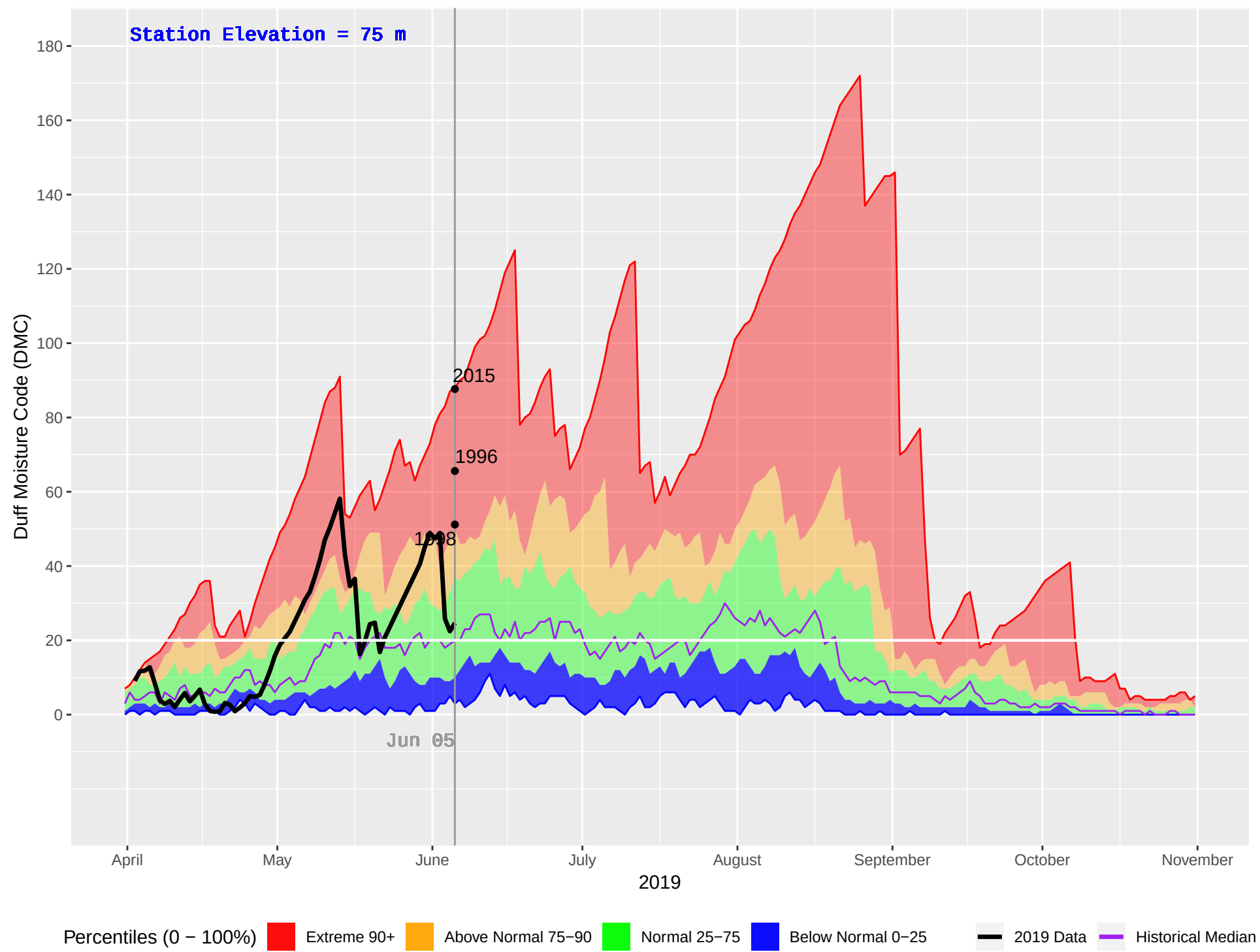
KITPARK (106) : Historical (1995–2018), Current (2019) Daily Duff Moisture Code (DMC)
