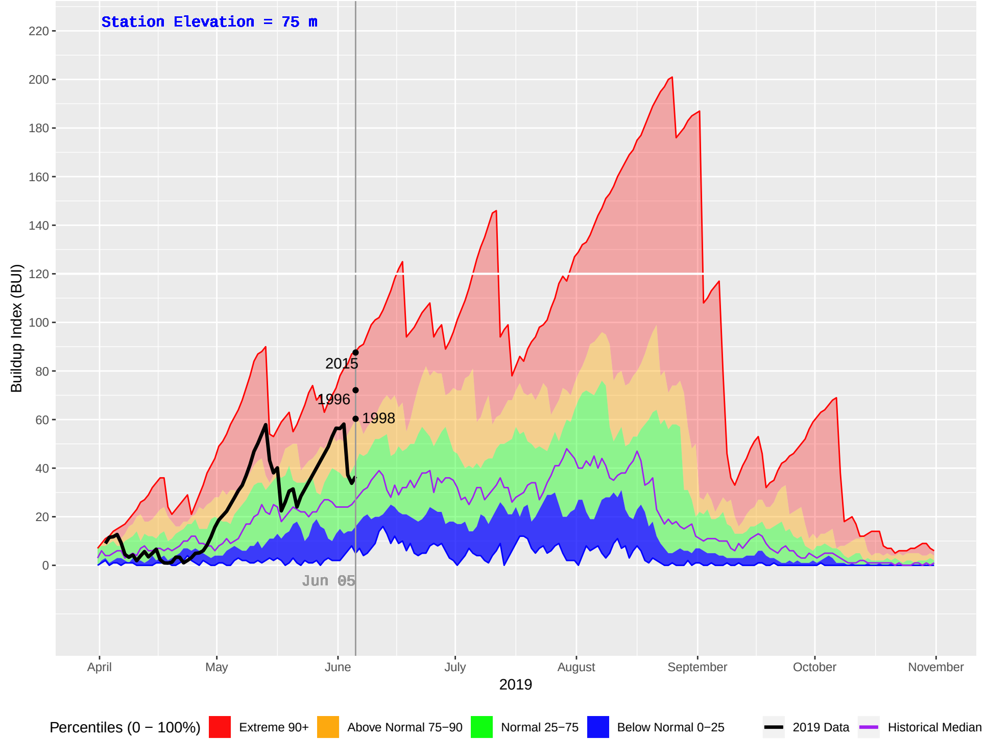
KITPARK (106) : Historical (1995–2018), Current (2019) Daily Buildup Index (BUI)
