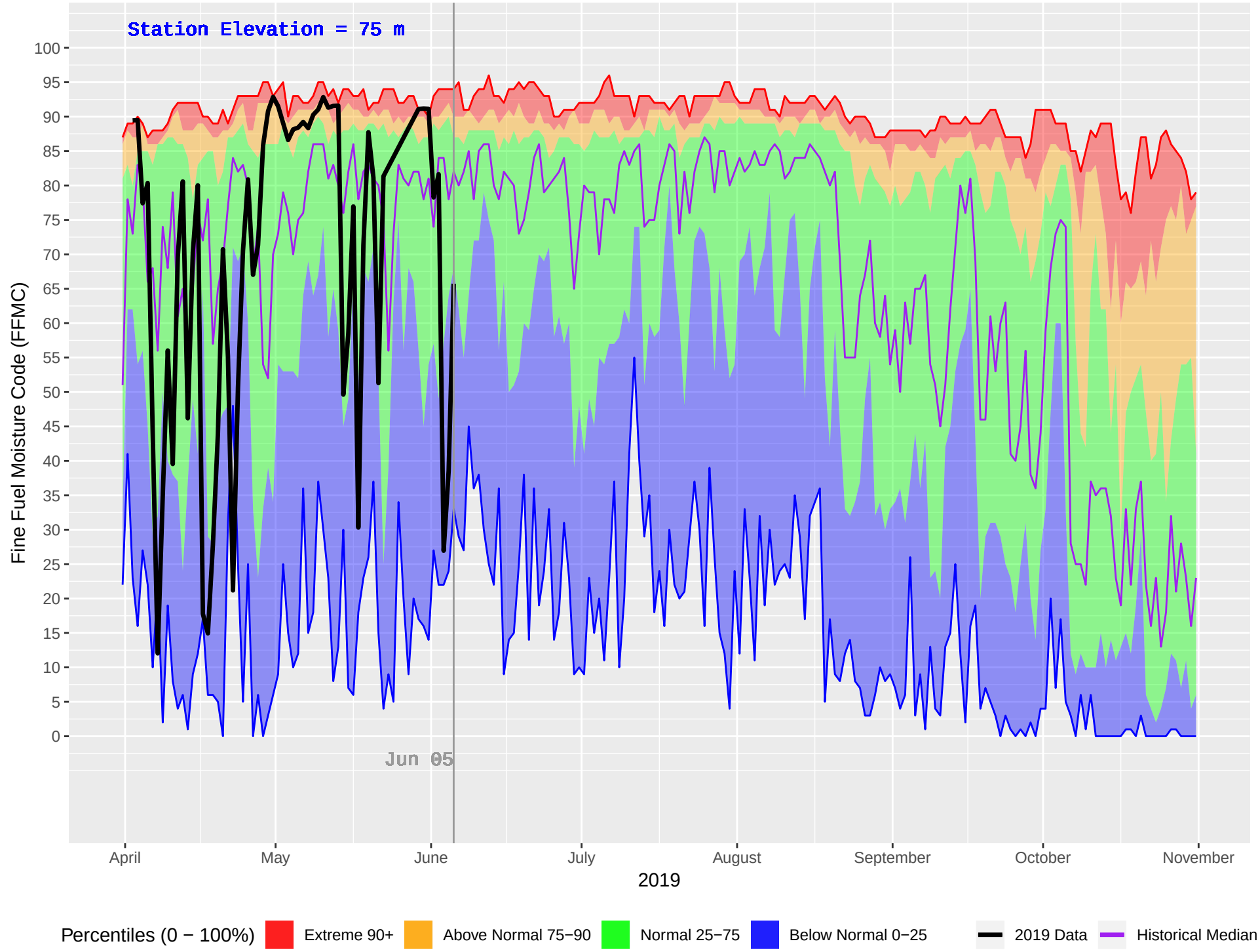
KITPARK (106) : Historical (1995–2018) and Current (2019) Daily Fine Fuel Moisture Code (FFMC)
