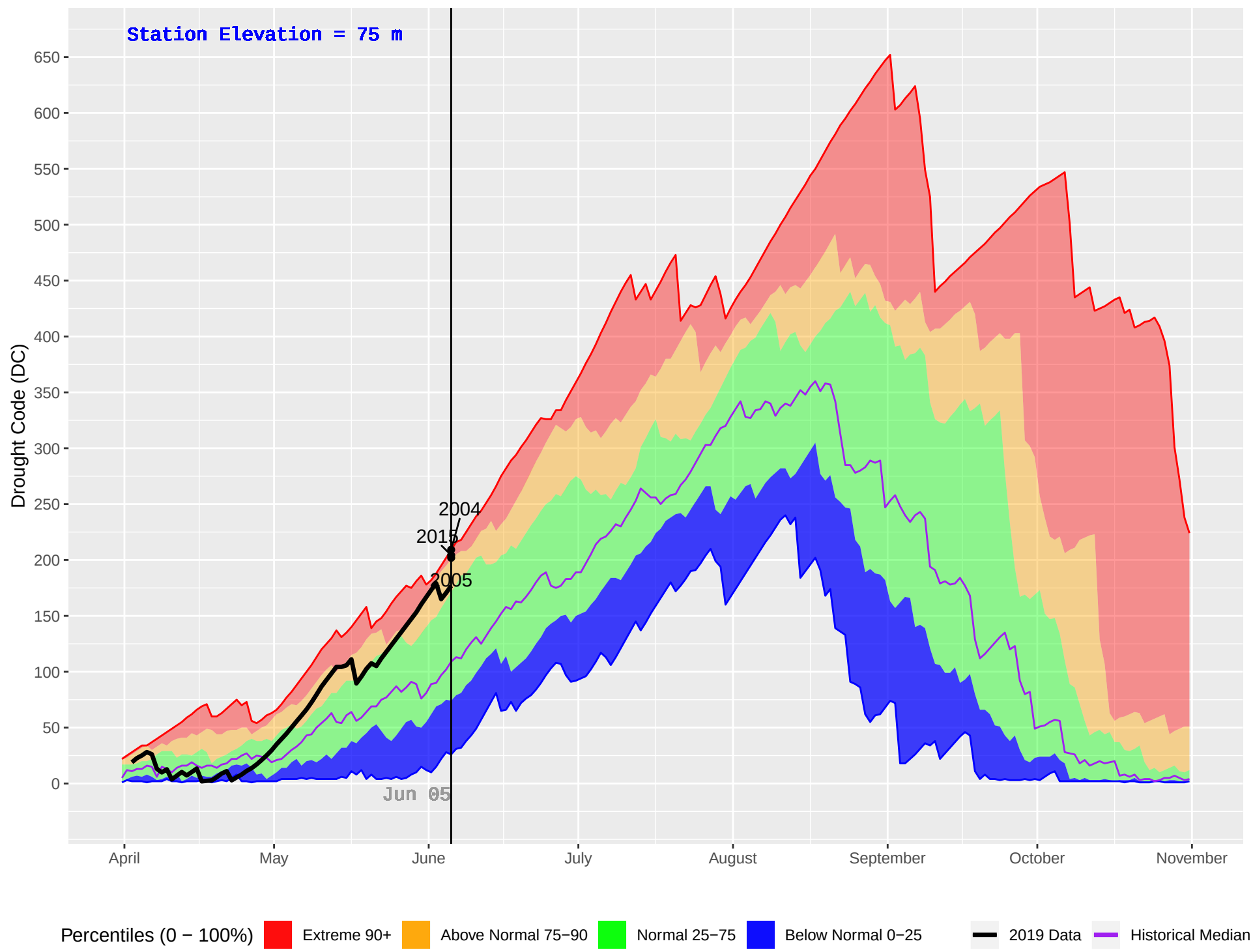
KITPARK (106) : Historical (1995–2018) and Current (2019) Daily Drought Code (DC)
